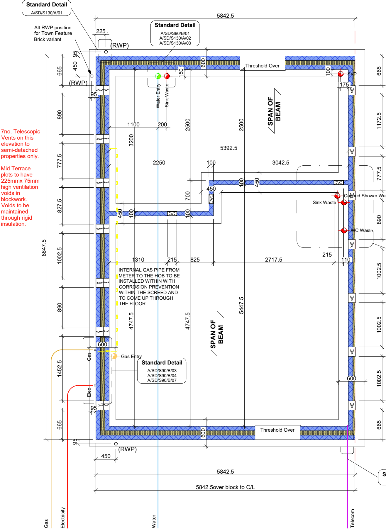
1 Foundation Plan with Semi Detached Service Entry Points 1 : 50
