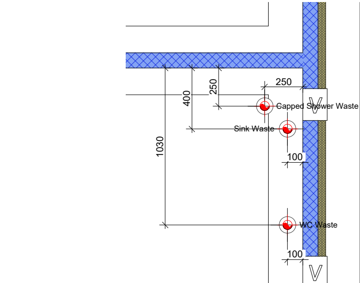
3 Ground Floor WC Drainage Callout 1 : 25
